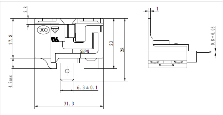
附图 5 Drawing 5 Overload Protector
