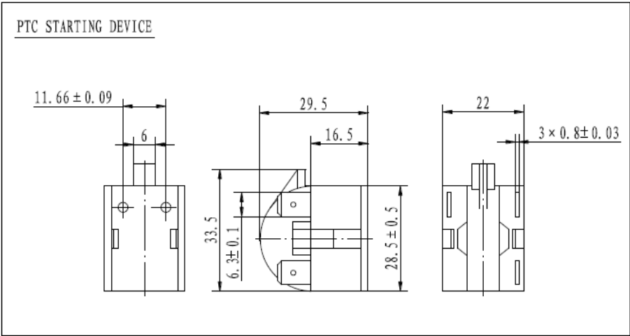
附图 4 Drawing 4 Starting Device
