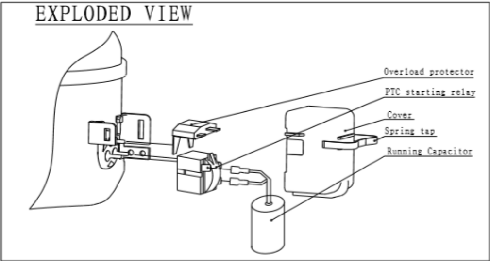
附图 2 Drawing 2 RSCR
